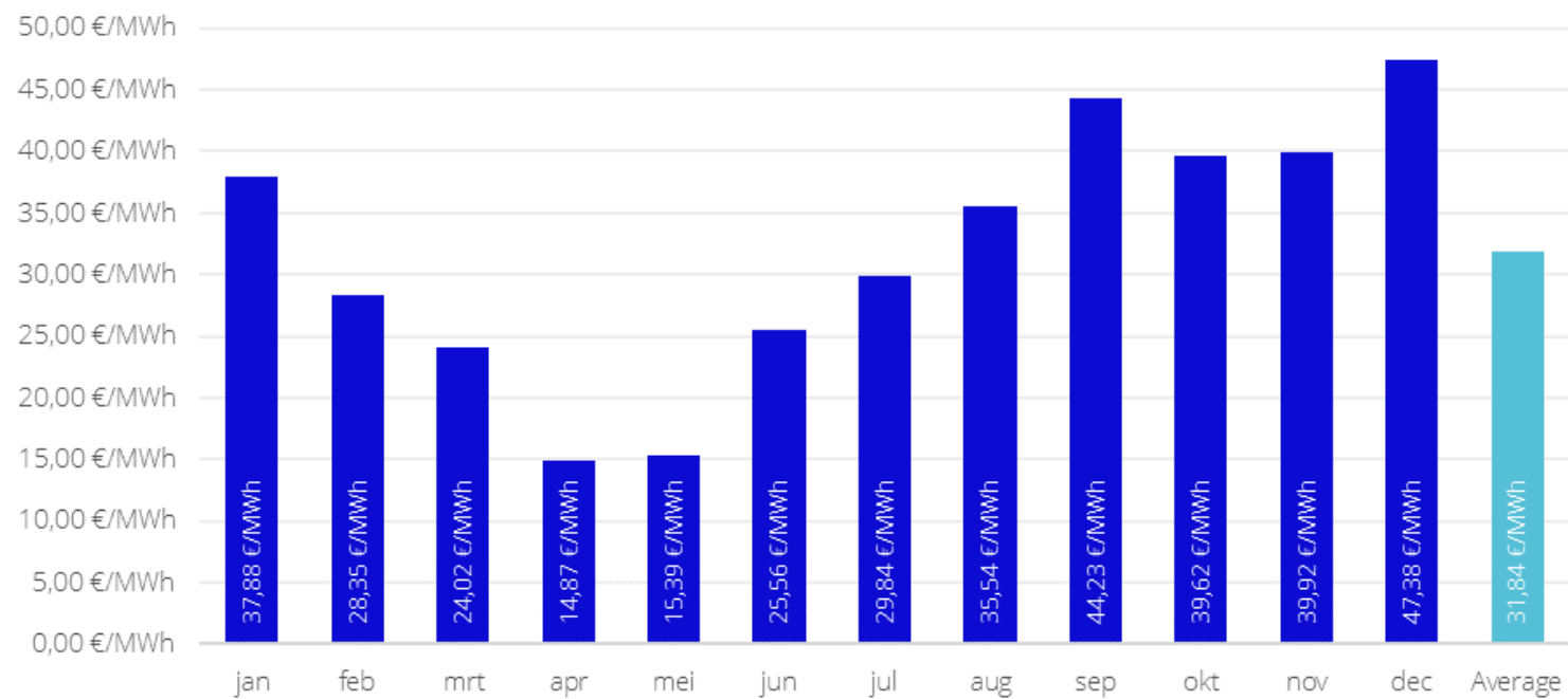
BELPEX AVERAGE 2020
